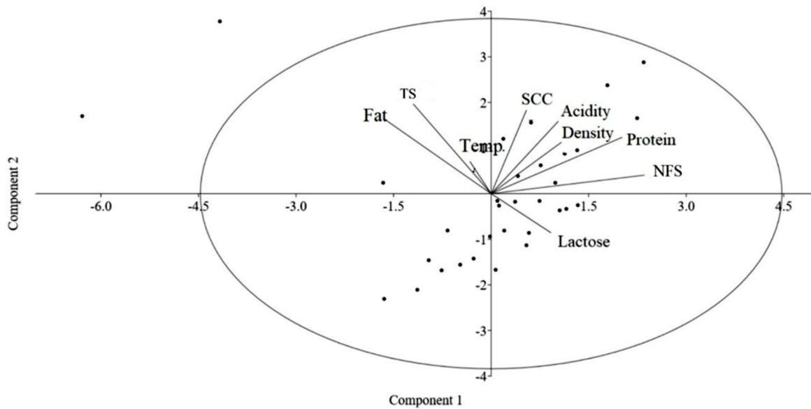
Figure 2. Ordination graphic about the multivariate analysis of the main components of the physicochemical parameters and milk composition of samples of refrigerated raw milk from dairy properties in Vale do Taquari - RS. TS: Total solids; NFS: Non-fat solids; Temp.: Temperature.
